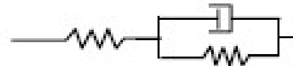
3-Parameter Solid
