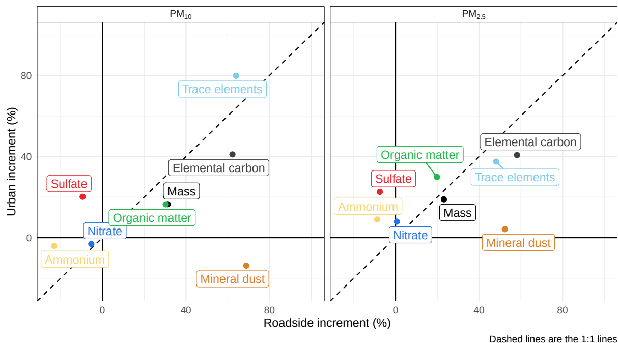
Figure 14 – Urban enrichment versus roadside enrichment of the mass concentration and the concentration of main chemical constituents in PM_{10} (left) and PM_{2.5} (right) for the 2018–2019 measurement period.
