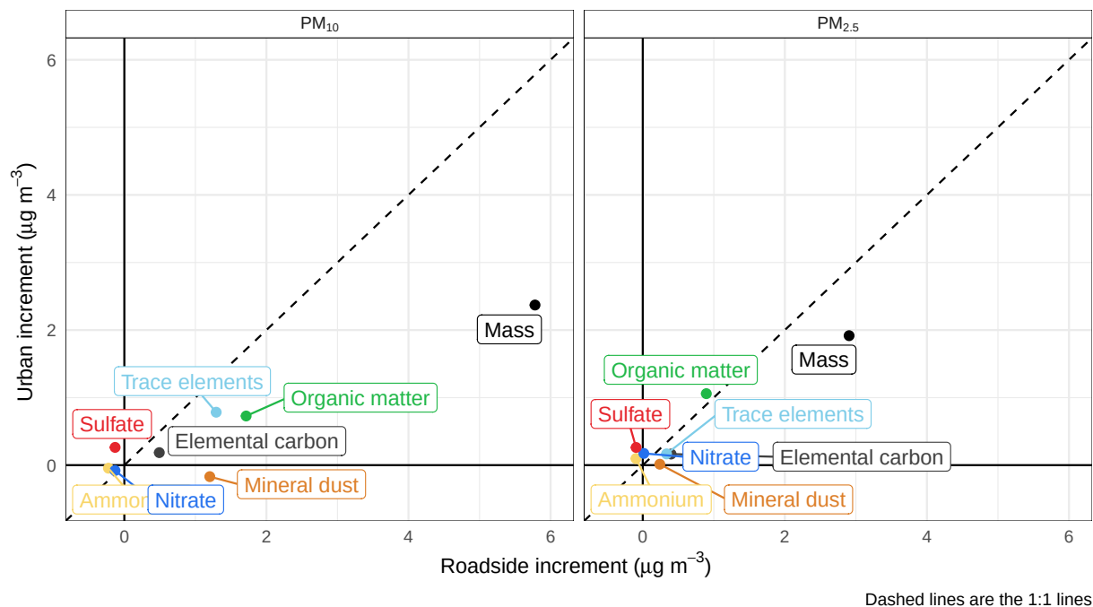
Figure 13 – Urban increment versus roadside increment of the mass concentration and the concentration of main chemical constituents in PM_{10} (left) and PM_{2.5} (right) for the 2018–2019 measurement periods. The urban increment was calculated from the concentration differences at the urban site Zürich-Kaserne and the rural site Payerne, whereas the roadside increment has been derived from the concentration differences at the urban roadside site Bern-Bollwerk and the urban site Zürich-Kaserne.
