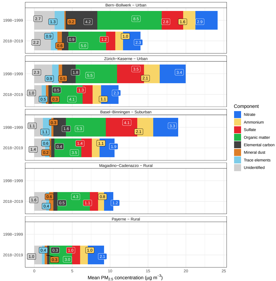
Figure 9 – Mean concentration of \text{PM}_{2.5} and the main chemical components \text{PM}_{2.5} for five monitoring sites in Switzerland for the duration of the field campaigns in 1998-1999 and 2018-2019. Note that \text{PM}_{2.5} was not included in the field campaign in 2008-2009.
