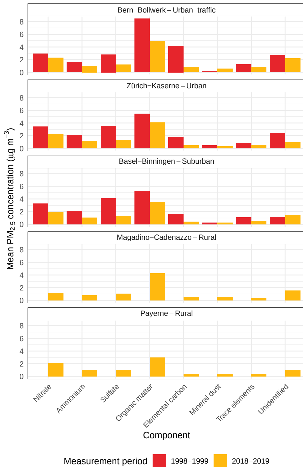
Figure A.8 – Mean concentrations of major constituents in PM 2.5 for the the 1998–1999 and 2018–2019 measurement periods.
