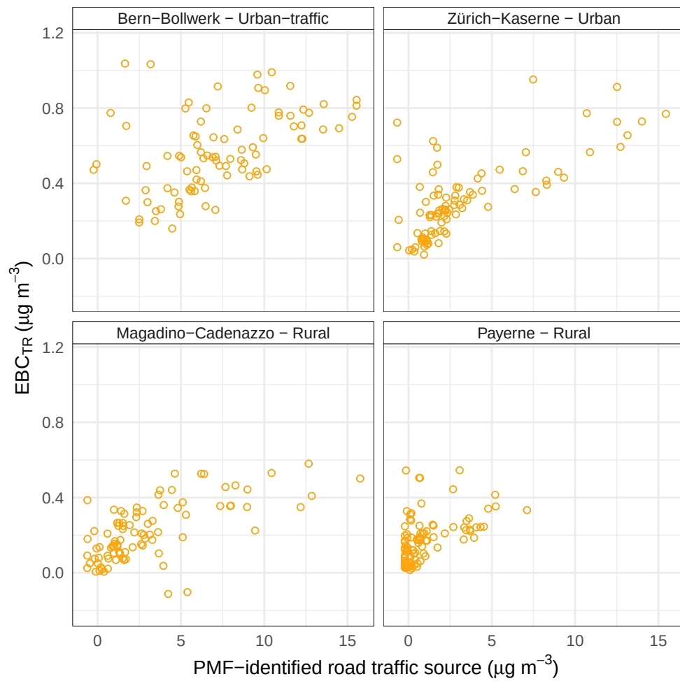
Figure A.20 – Scatterplots of traffic equivalent black carbon (EBC TR ) and the PMF-identified road traffic sources at four Swiss sites between 2018 and 2019.
