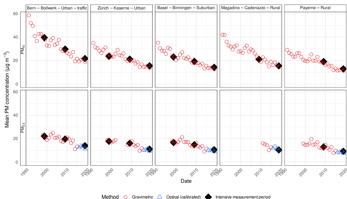
Figure 20 – Annual PM 10 and PM 2.5 means for five monitoring sites in Switzerland between 1991 and 2019. The different open symbols indicate a change in measurement method from gravimetric to an optical method that is corrected based on regular parallel measurements with the gravimetric method.
