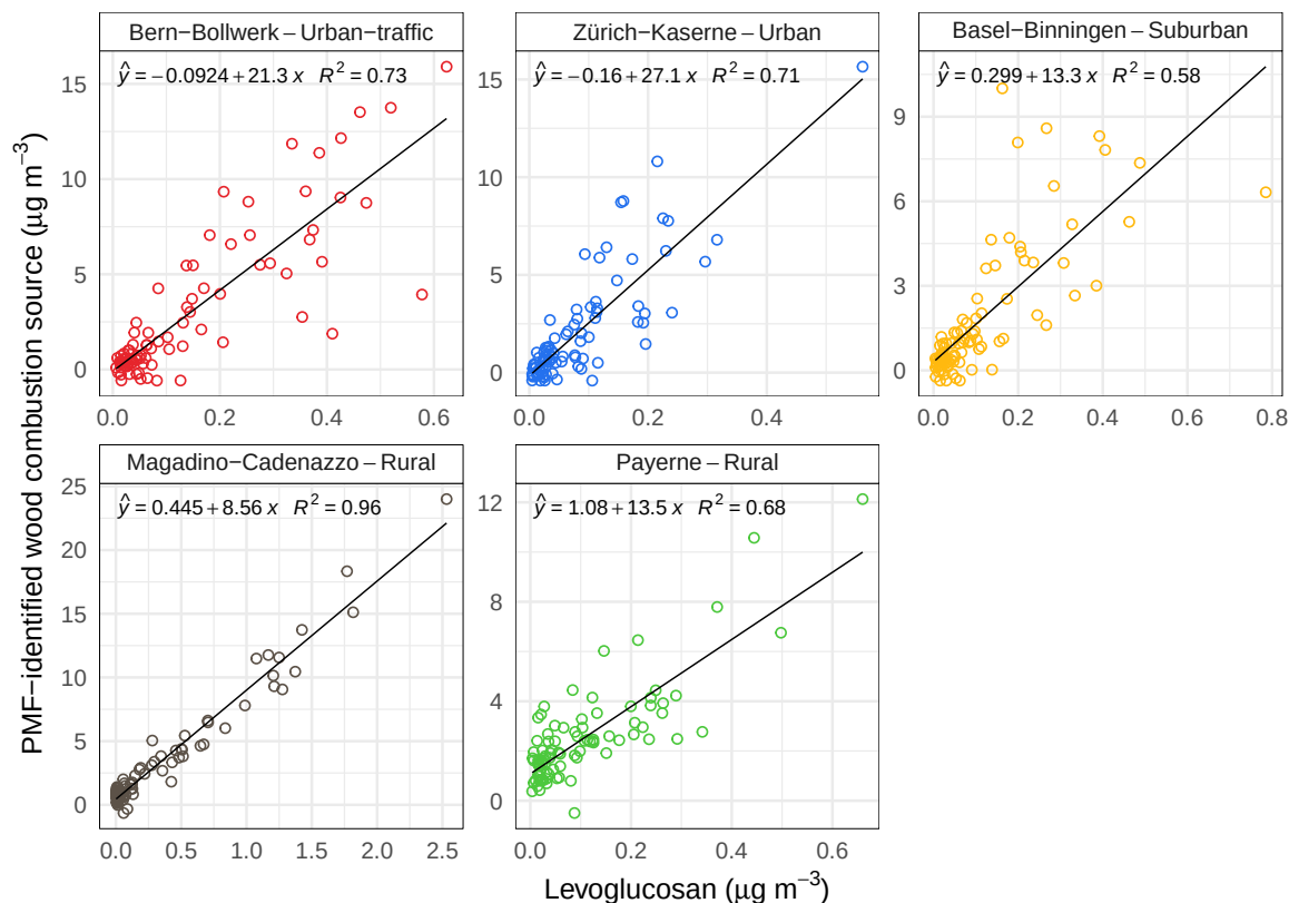
Figure 25 – Contribution of the wood combustion sources to PM 10 versus levoglucosan for five sites in Switzerland between 2018 and 2019.
