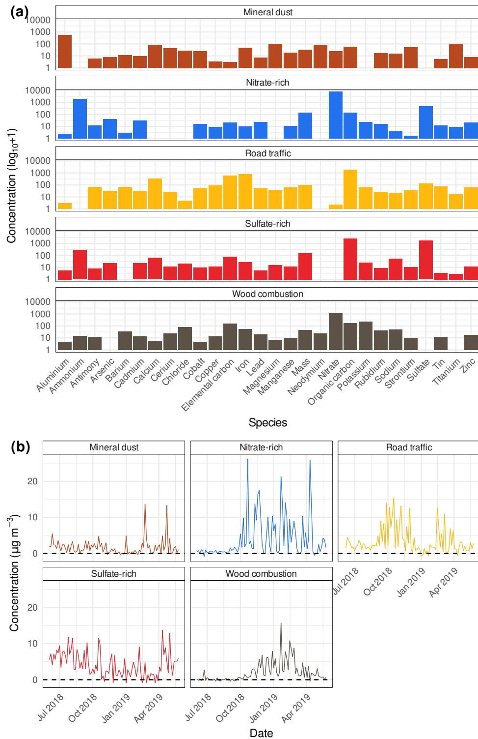
Figure A.13 – Zürich-Kaserne \text{PM}_{10} source contributions (a) and time series (b) between June 1, 2018 and May 31, 2019 identified by positive matrix factorisation (PMF).
