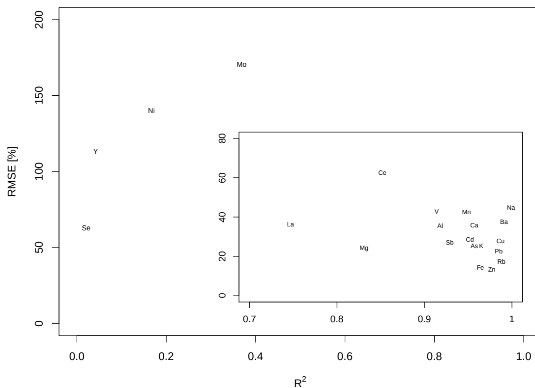
Figure A.1 – Comparison of the results of two different analytical procedures for determination of element concentrations in PM. PM 10 filter samples from Zürich-Kaserne and Payerne from 04.02.2009, 28.02.2009, 09.04.2009 and 02.07.2009 were analysed by Empa and IDAEA-CSIC using the analytical procedures as for the measurement periods 1998–1999 and 2008–2009 (Empa) and the recent measurement period 2018–2019 (IDAEA-CSIC). Shown is the root mean squared error (RMSE) divided by the mean element concentration versus the coefficient of determination ( R^2 ) for all elements in this method comparison. Few elements show a poor agreement with R^2 < 0.4 , however, most of the elements show a high correlation as shown by the inserted subplot.
