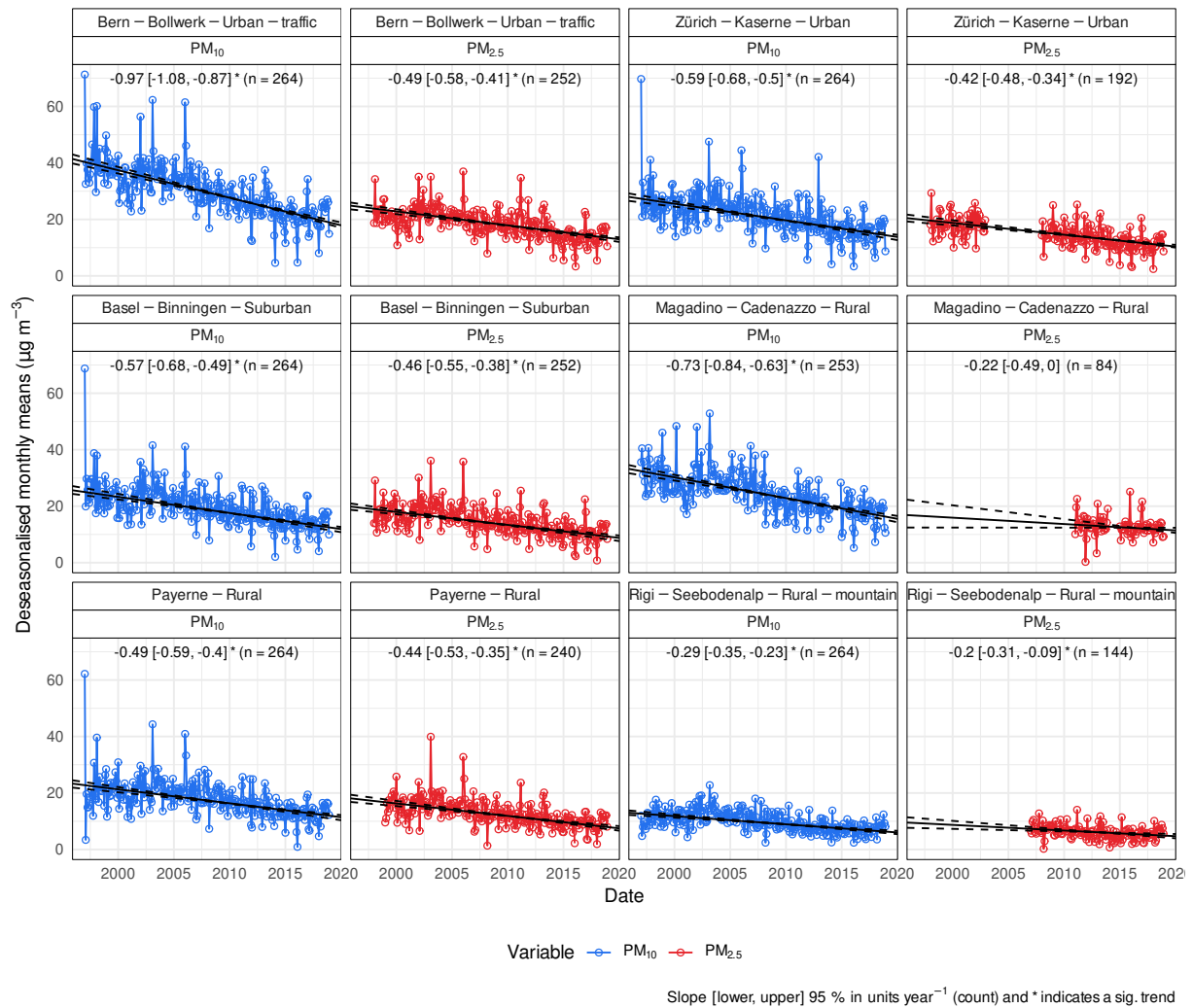
Figure 5 – PM 10 and PM 2.5 deseasonalised monthly means and trends for six monitoring locations in Switzerland between 1997 and 2020.
