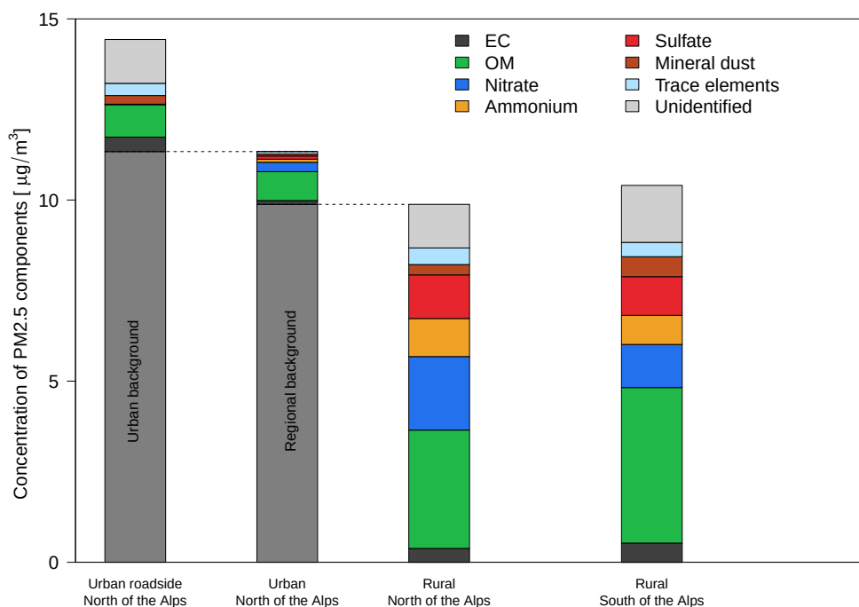
Figure 18 – Summary of mean chemical composition of PM_{2.5} for the 2018–2019 measurement period at a rural site south of the Alps (Magadino-Cadenazzo) and at regional background sites north of the Alps (mean of suburban site Basel-Binningen and rural site Payerne). The composition of the urban increment and the roadside increment as derived from the chemical composition data from Zürich-Kaserne and Bern-Bollwerk respectively is also shown.
